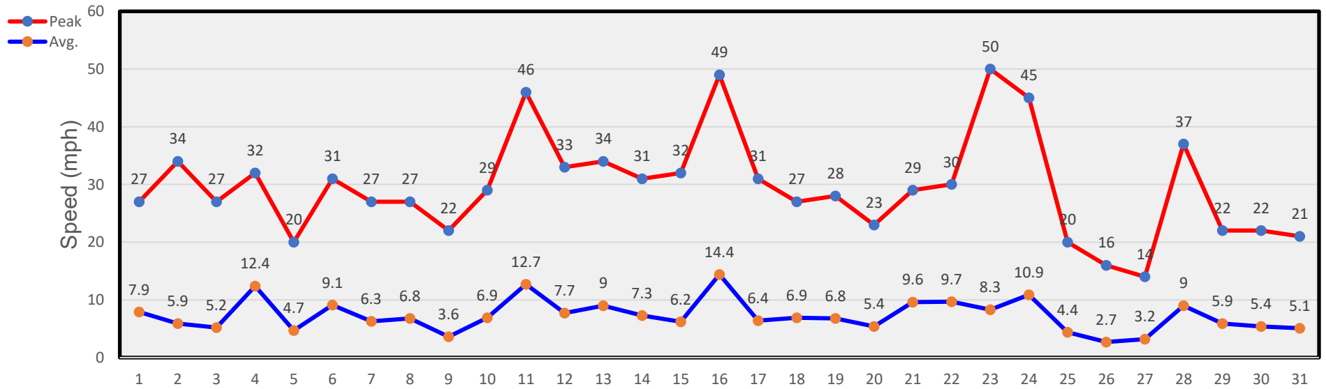
October Winds
