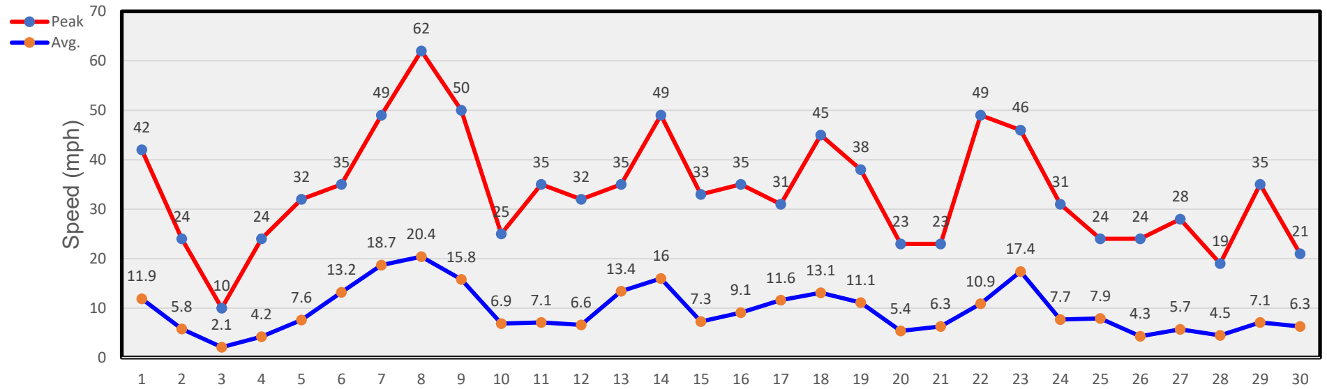
November Winds
