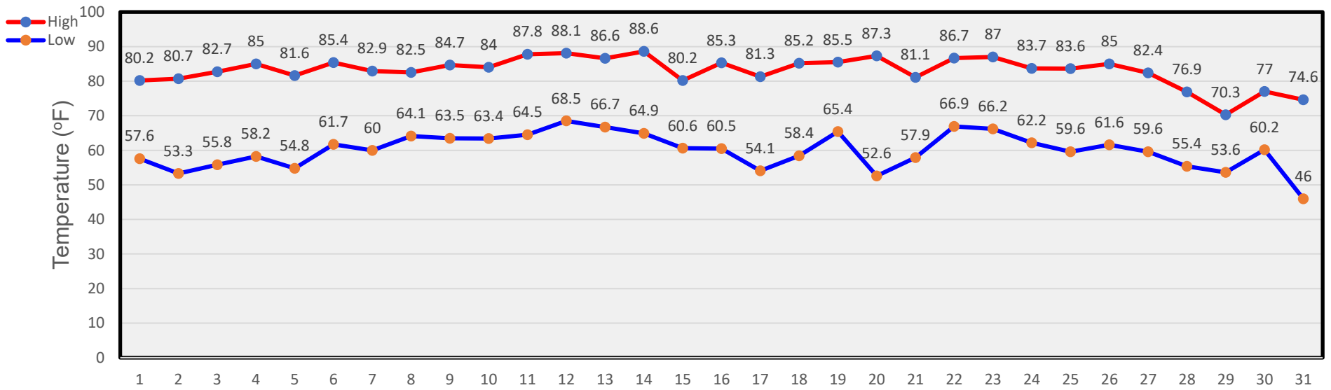
August Temperatures
