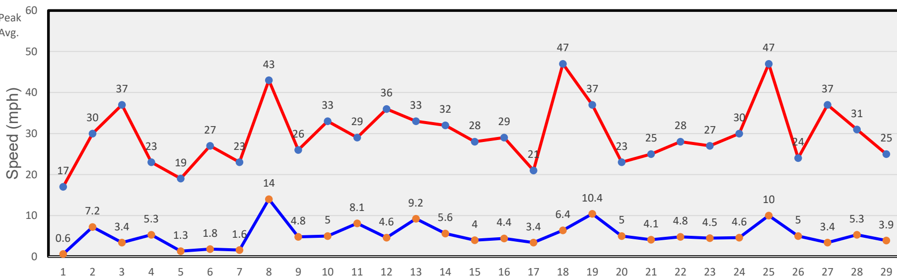
February Winds
