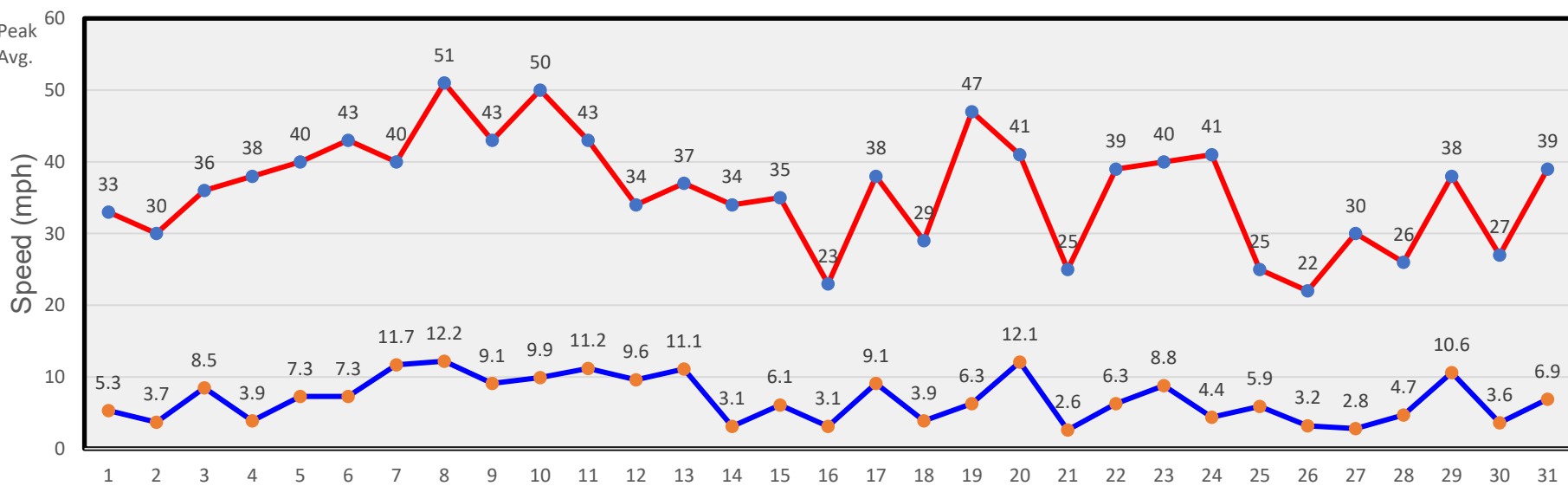
May Winds
