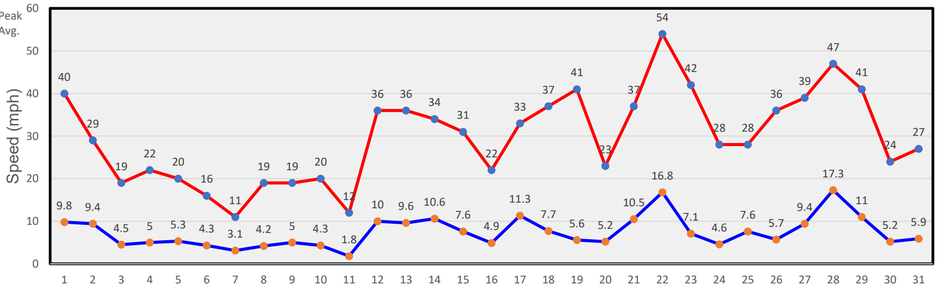
December Winds
