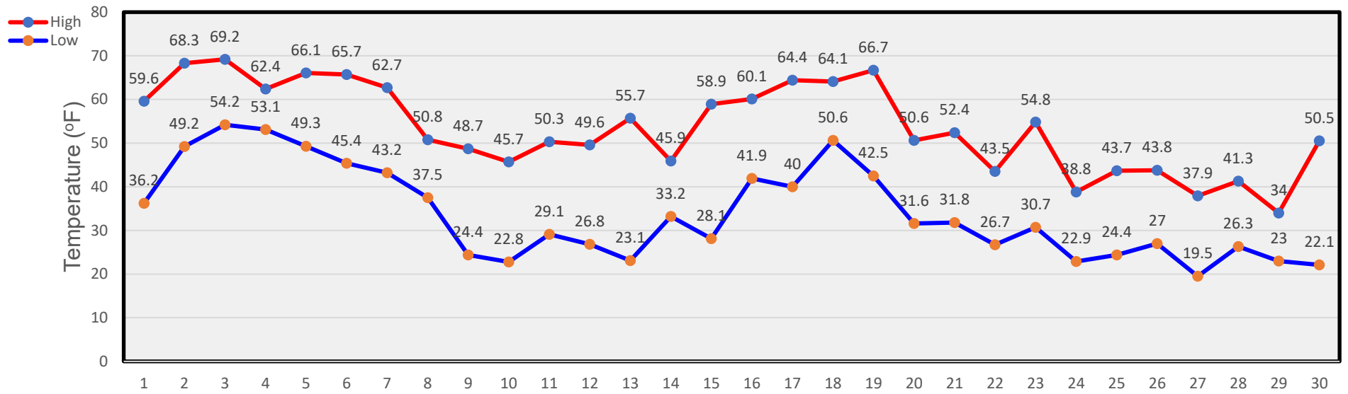
November Temperatures
