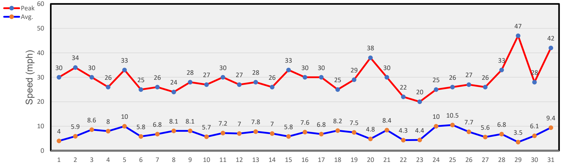
August Winds
