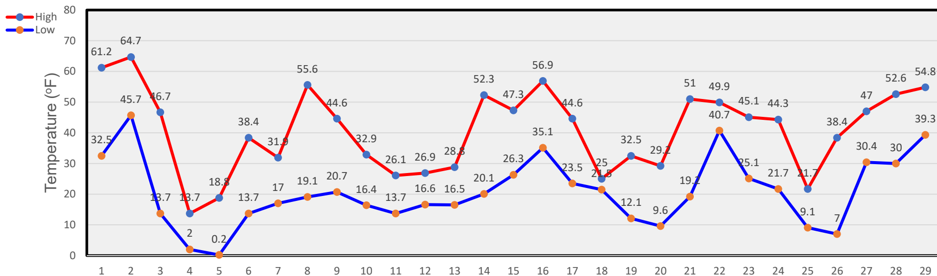
February Temperatures
