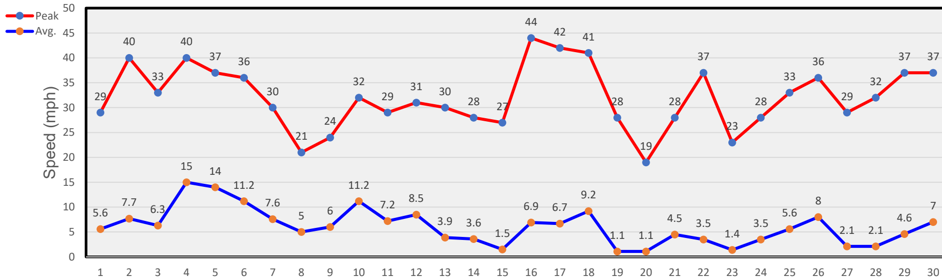
April Winds
