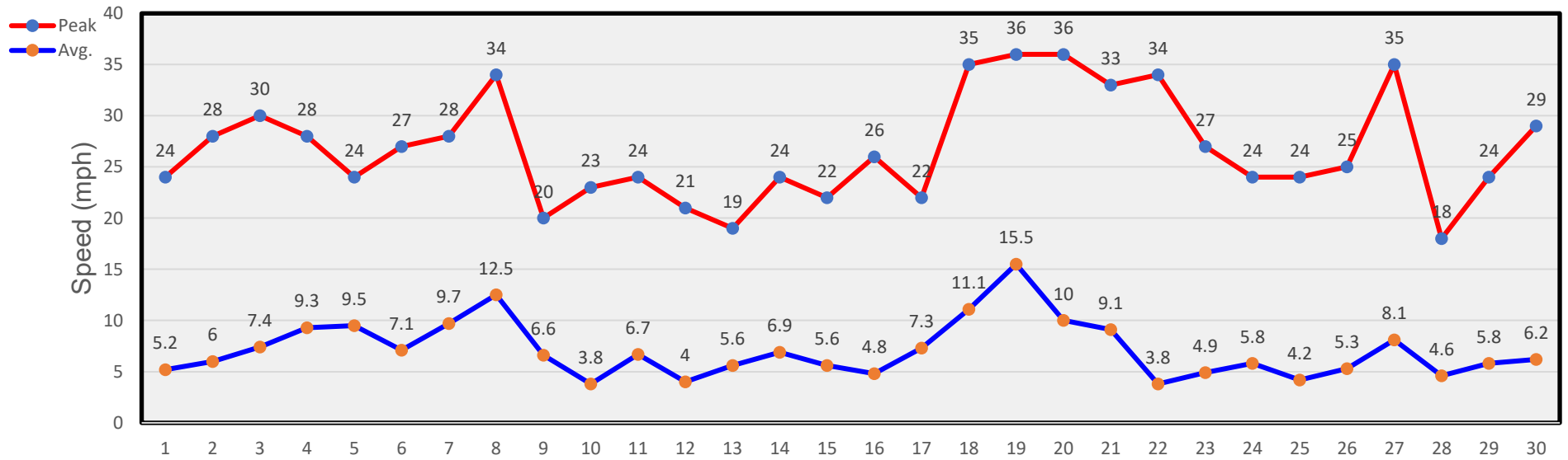
September Winds
