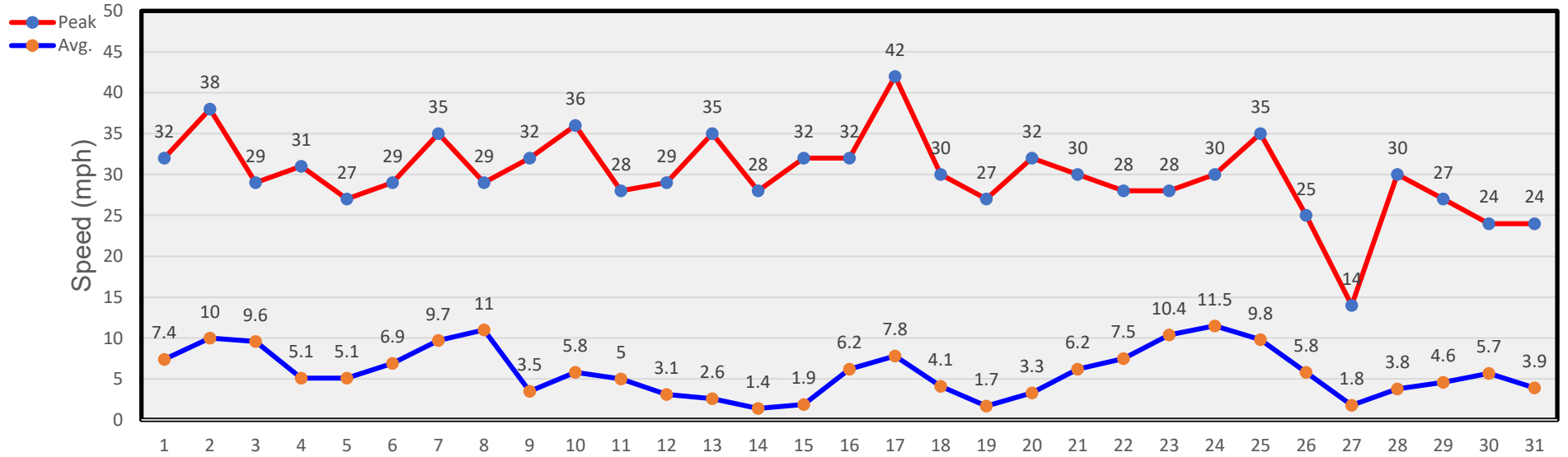
July Winds
