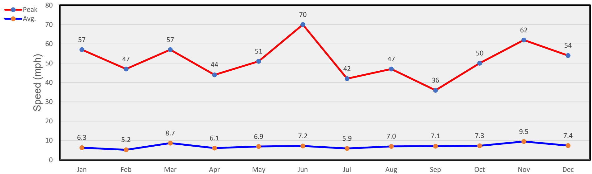
Monthly Winds
