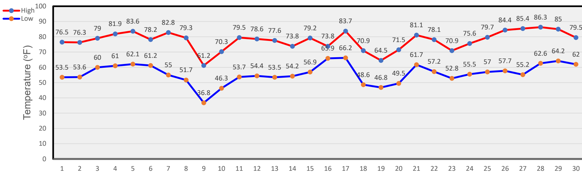
June Temperatures
