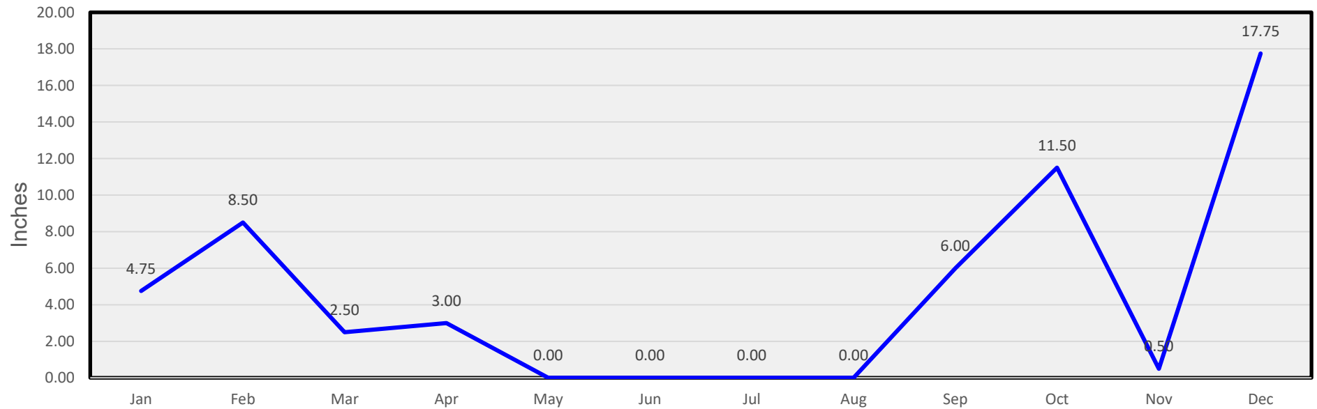
Monthly Snow
