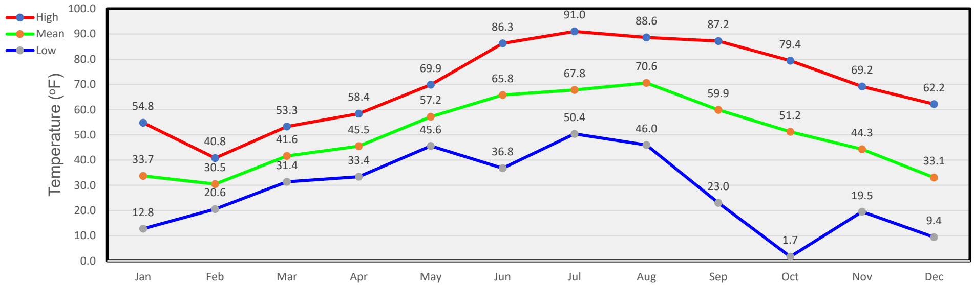
Monthly Temperatures
