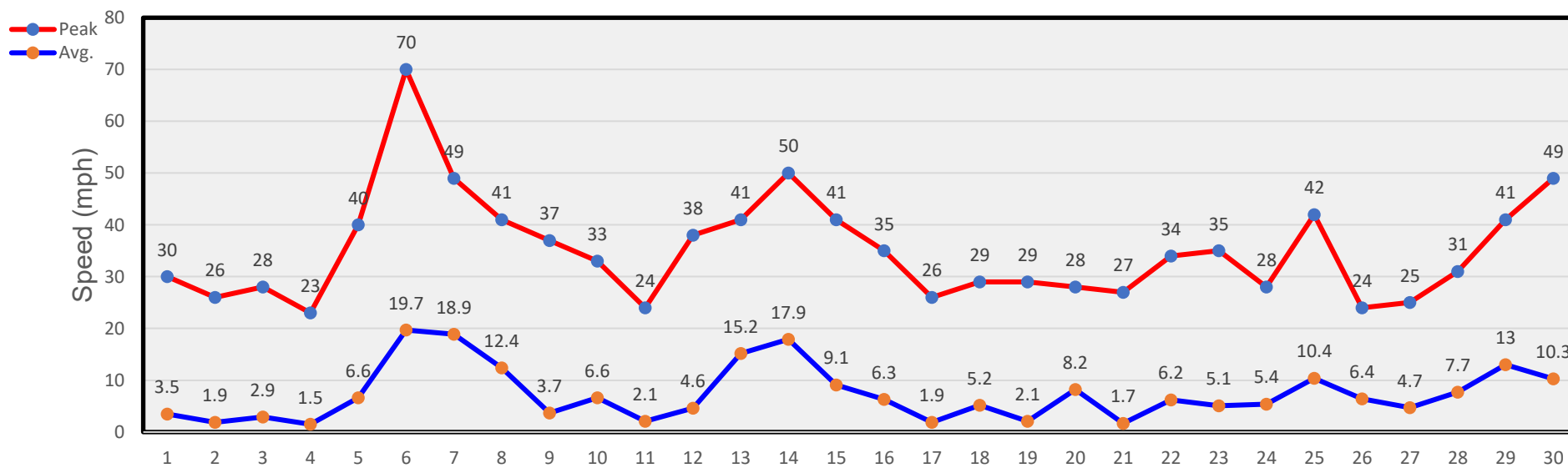
June Winds
