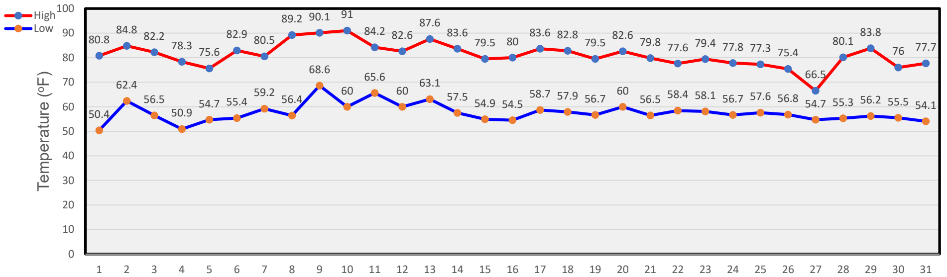
July Temperatures
