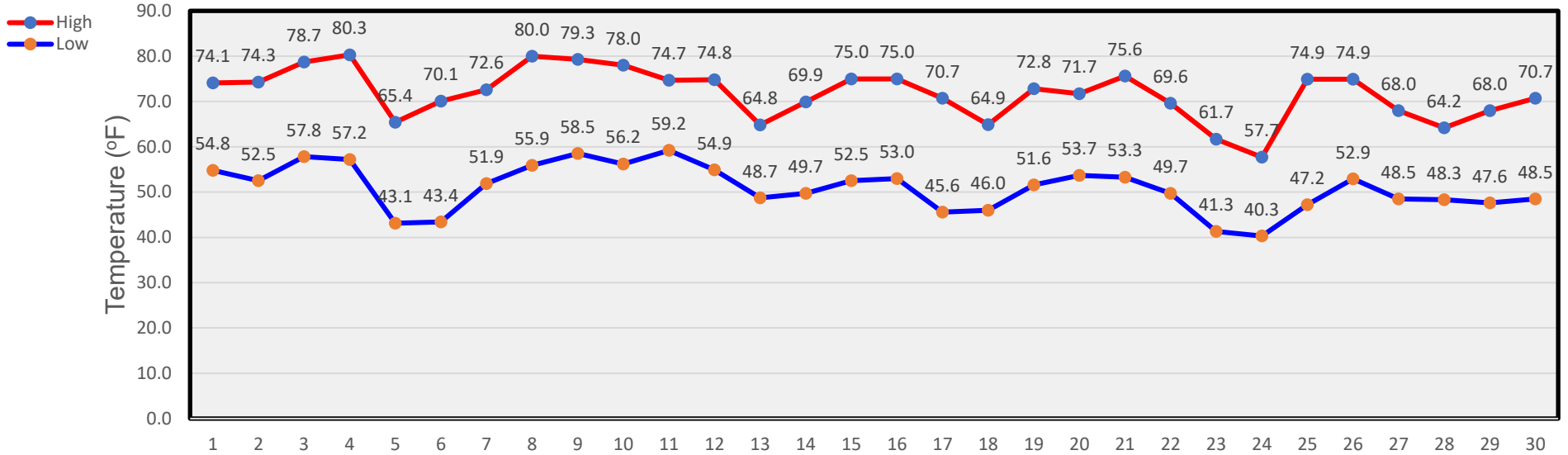
September Temperatures
