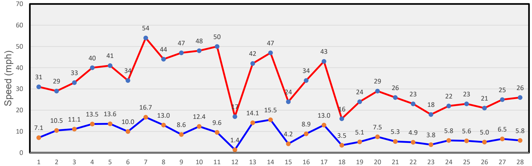
February Winds
