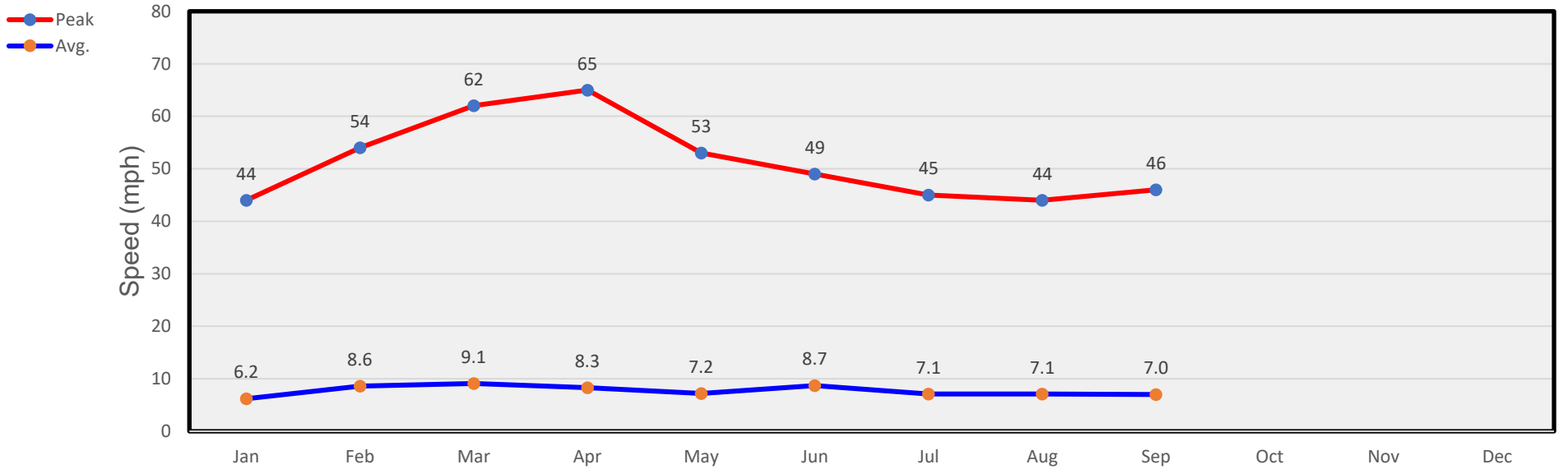
Monthly Winds
