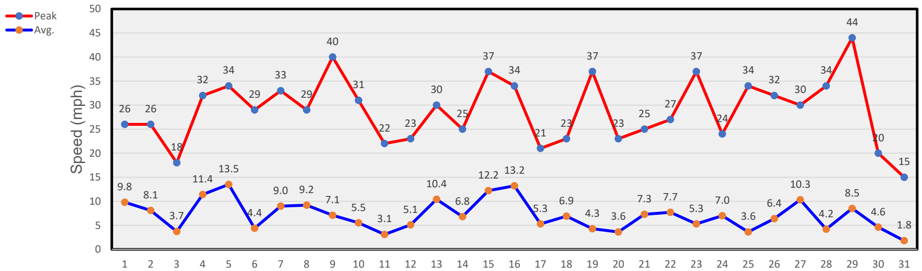
August Winds
