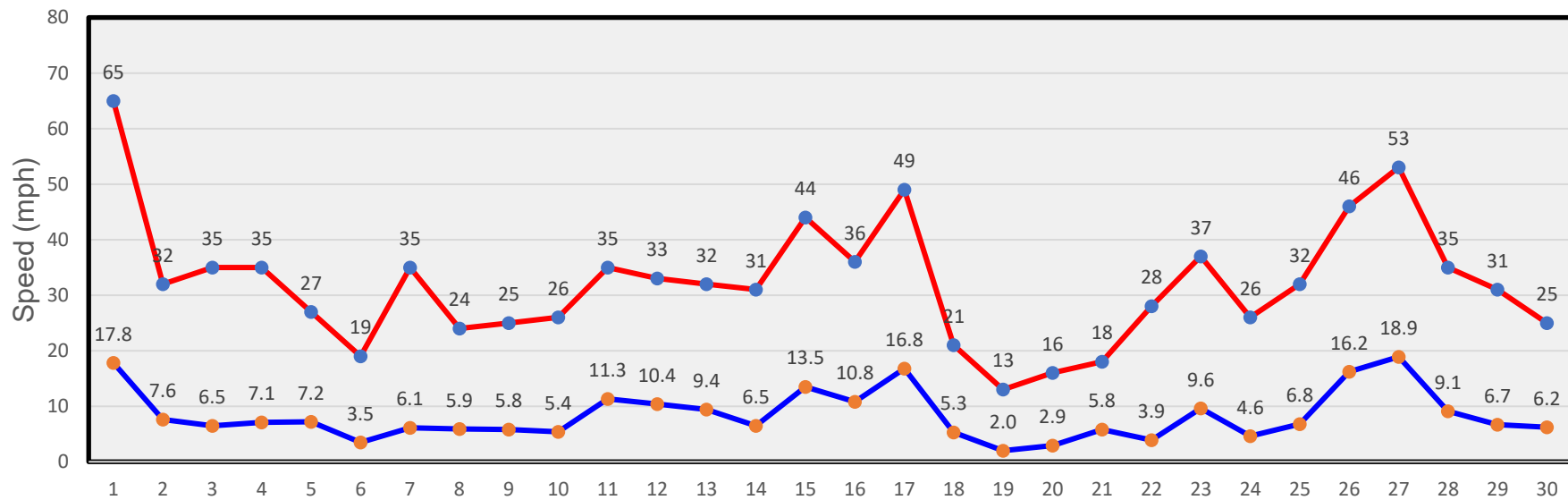
April Winds
