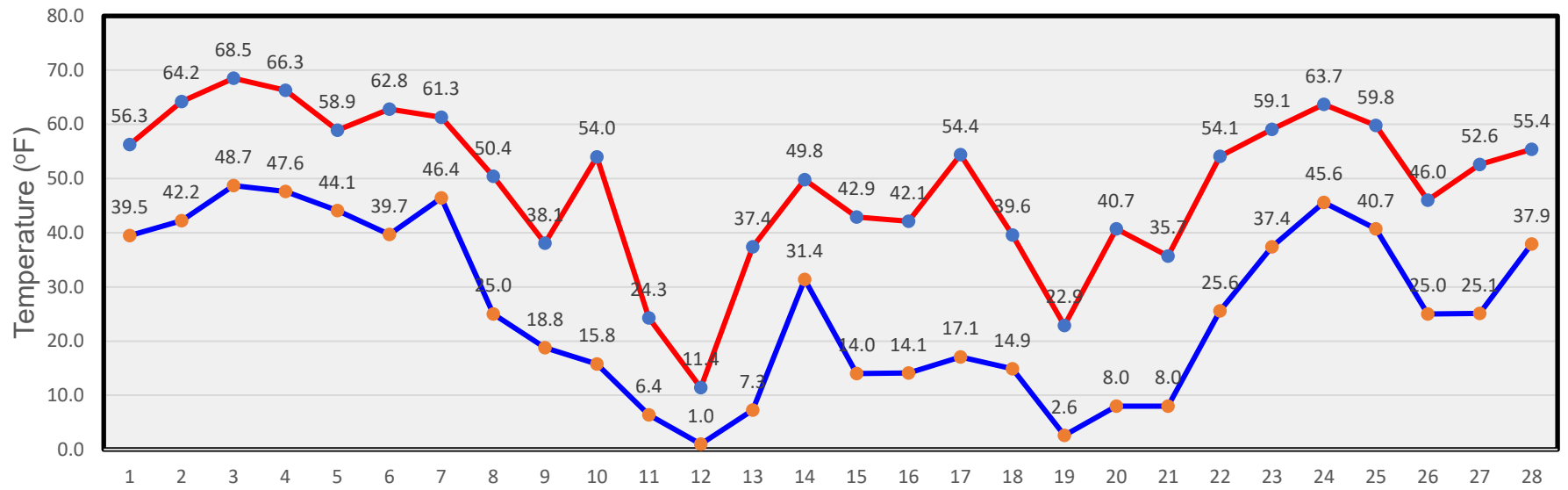
February Temperatures
