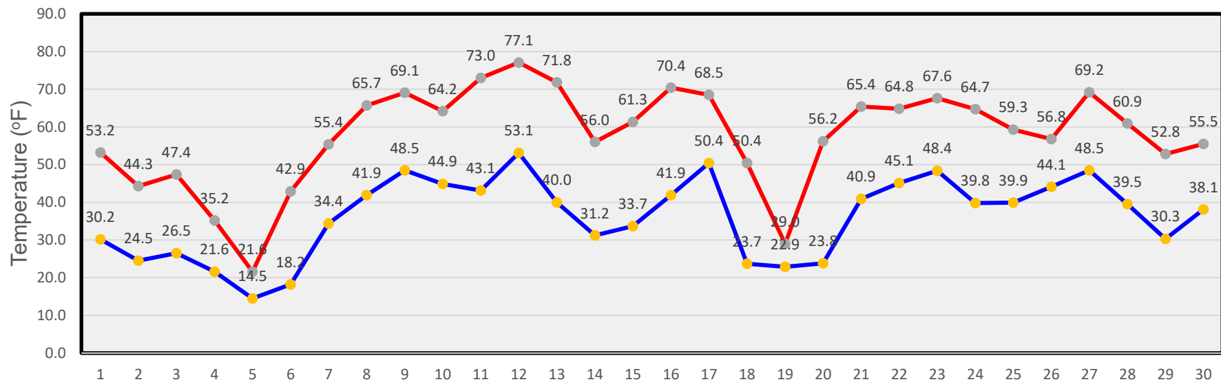
April Temperatures
