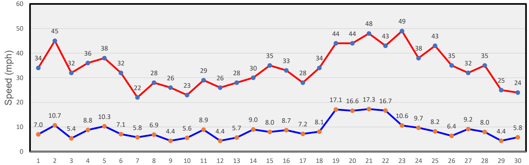
June Winds
