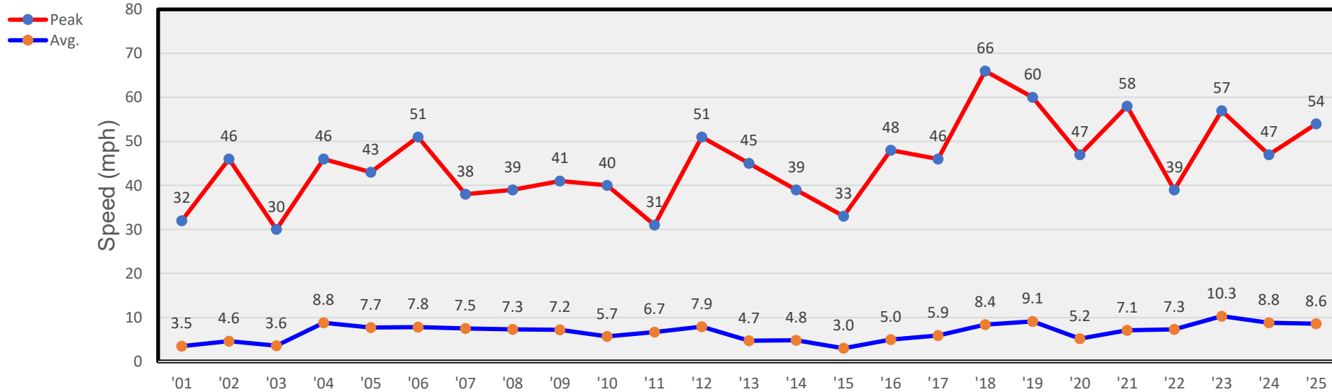
February Winds
