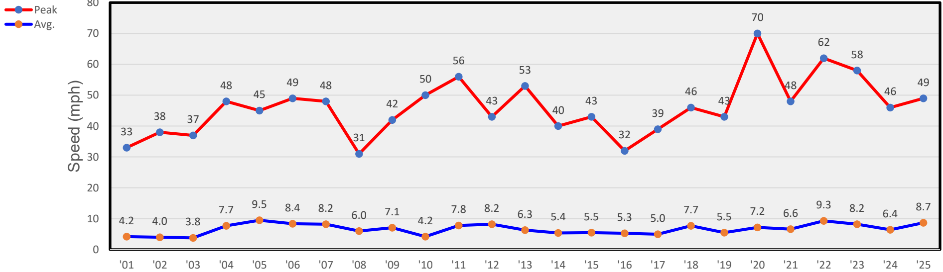
June Winds
