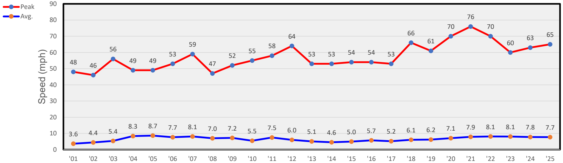
Yearly Winds
