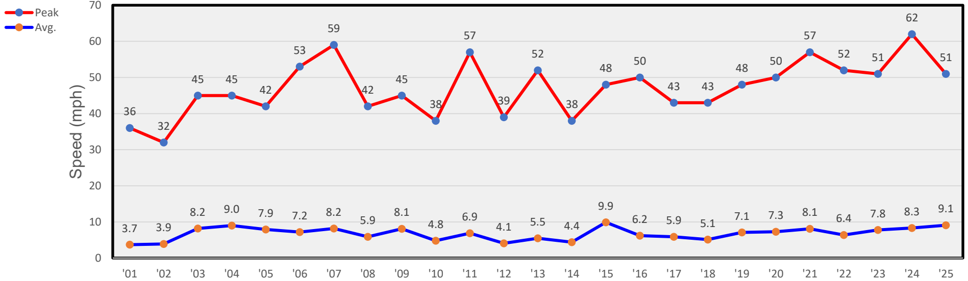
October Winds
