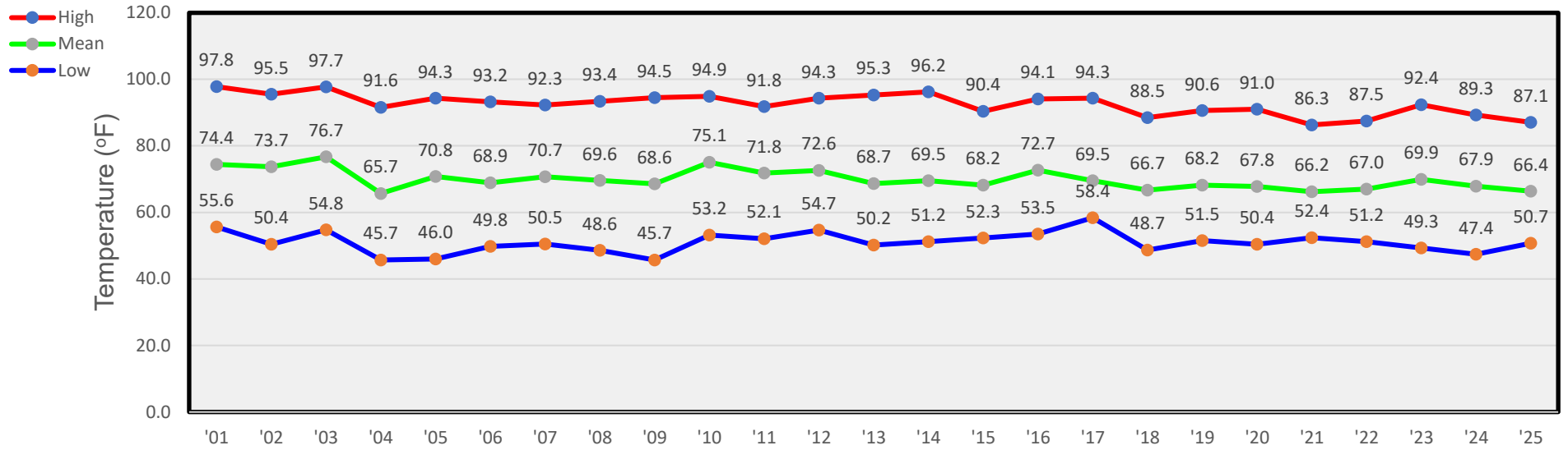
July Temperatures
