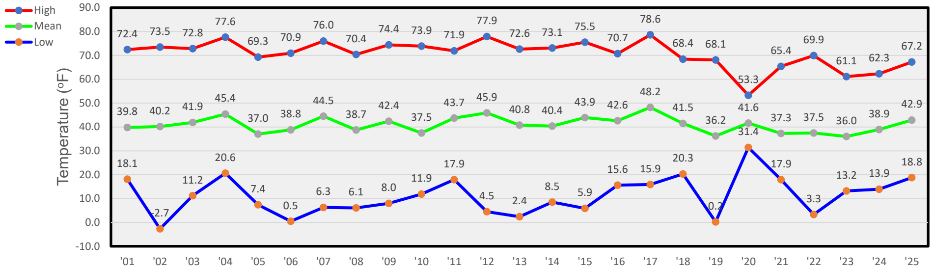
March Temperatures
