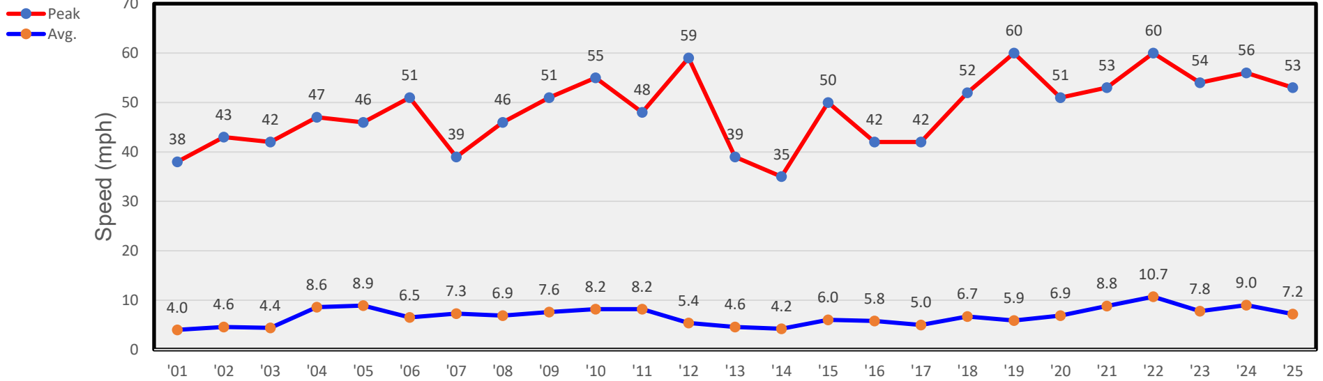
May Winds
