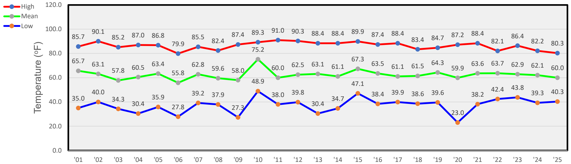
September Temperatures
