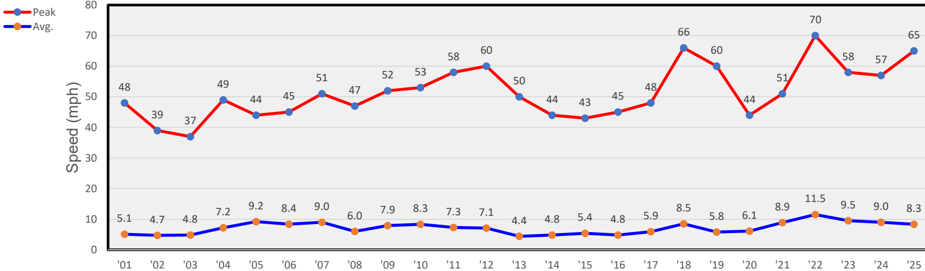
April Winds
