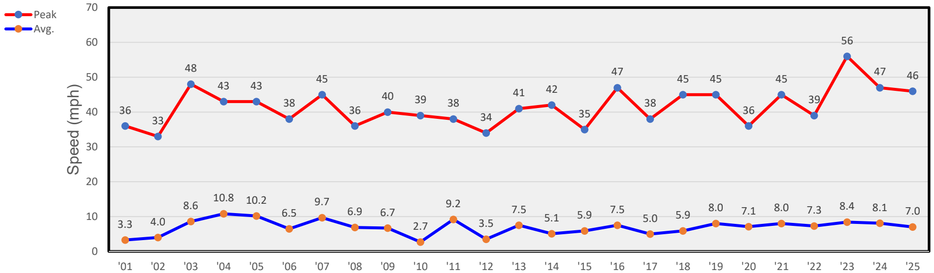
September Winds
