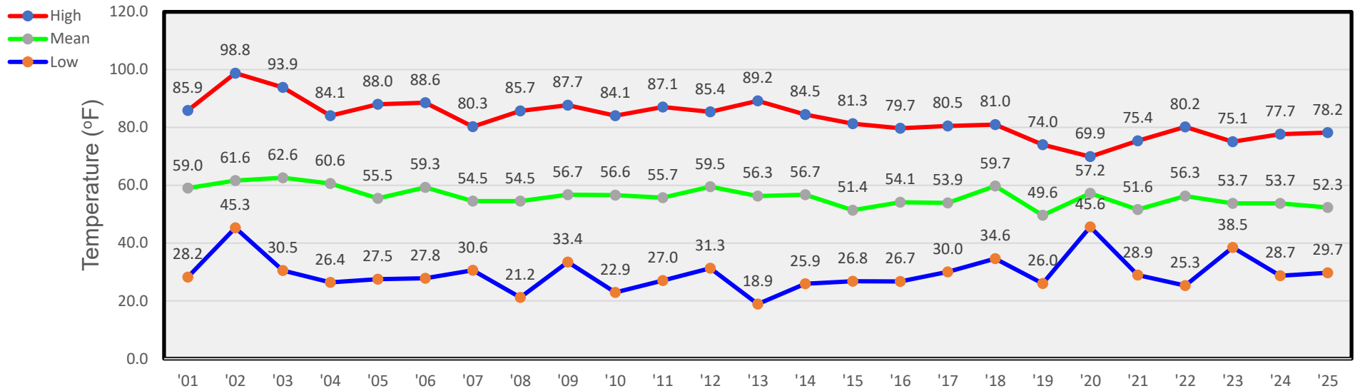
May Temperatures
