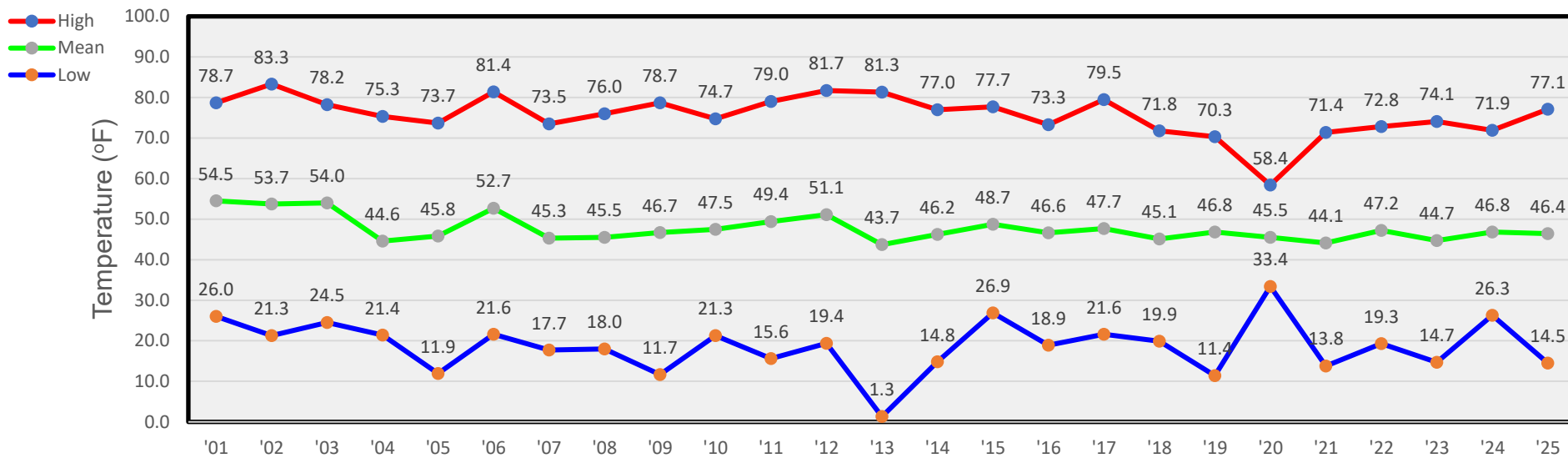
April Temperatures
