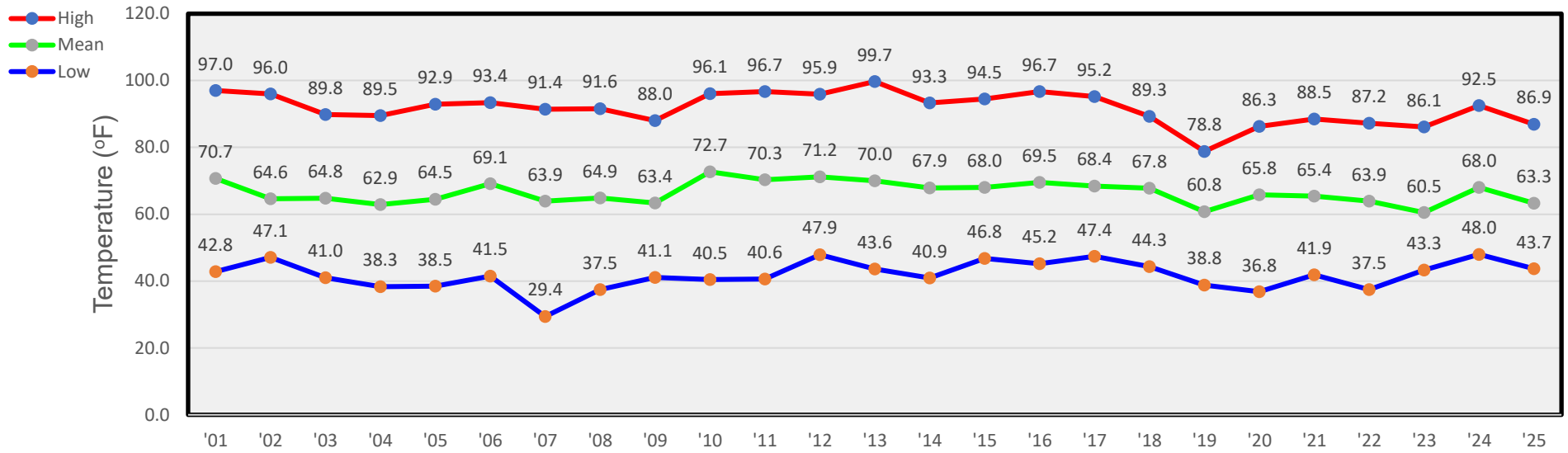
June Temperatures
