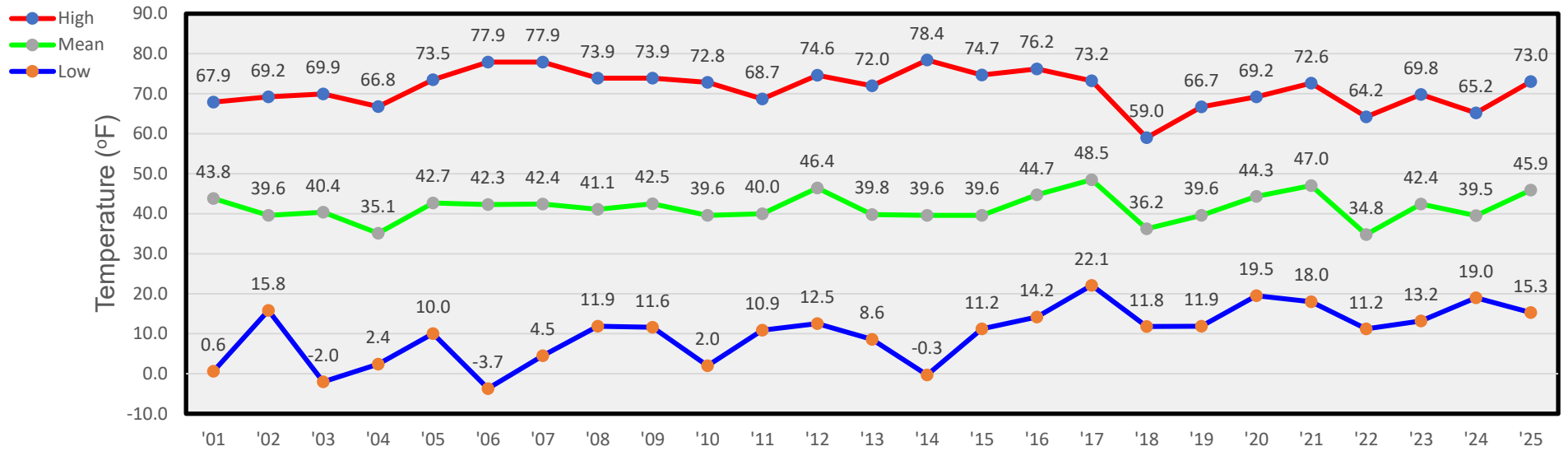
November Temperatures
