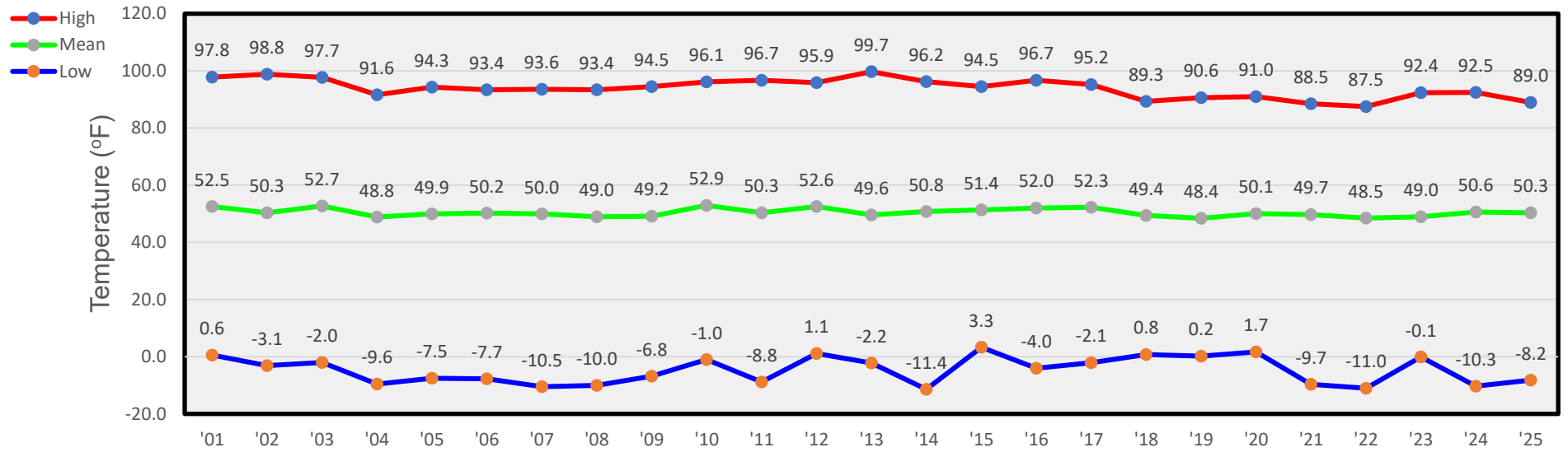
Yearly Temperatures
