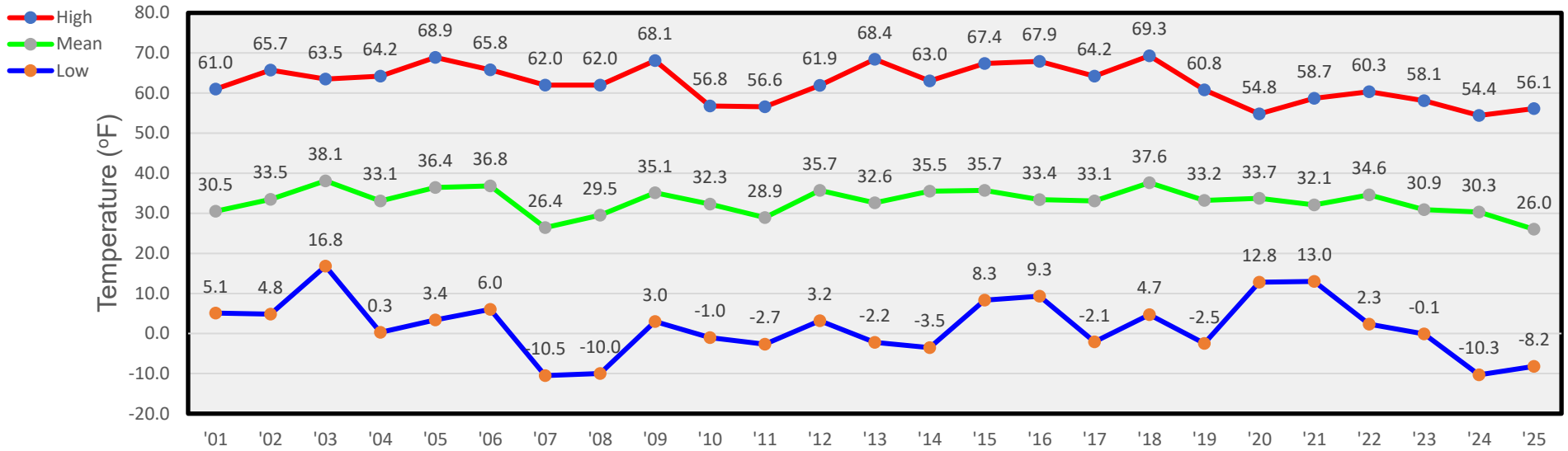
January Temperatures
