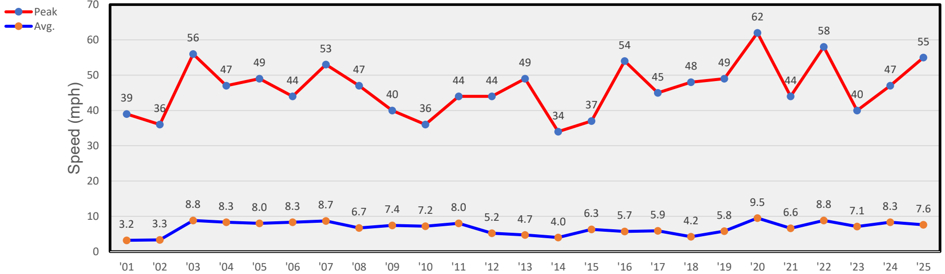
November Winds
