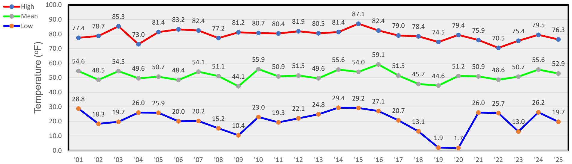
October Temperatures
