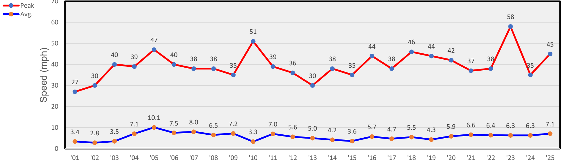
July Winds
