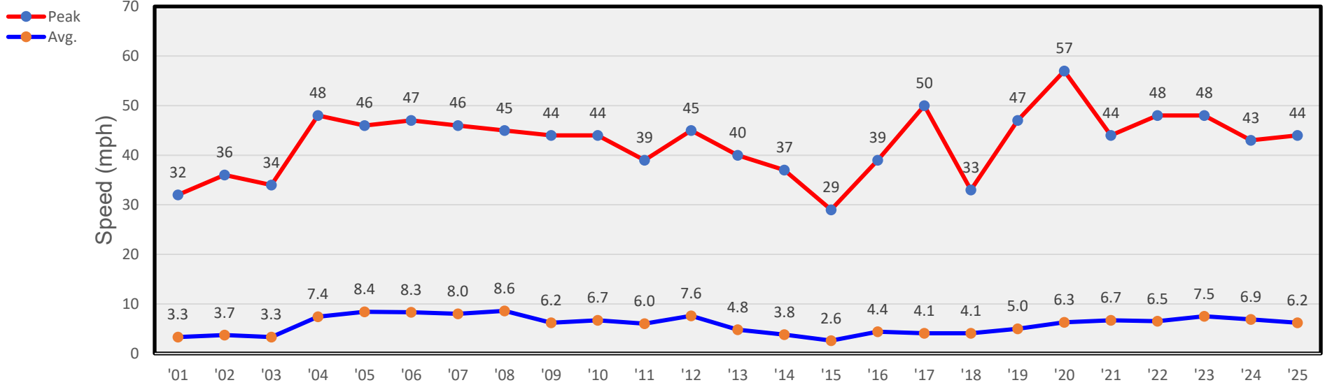
January Winds
