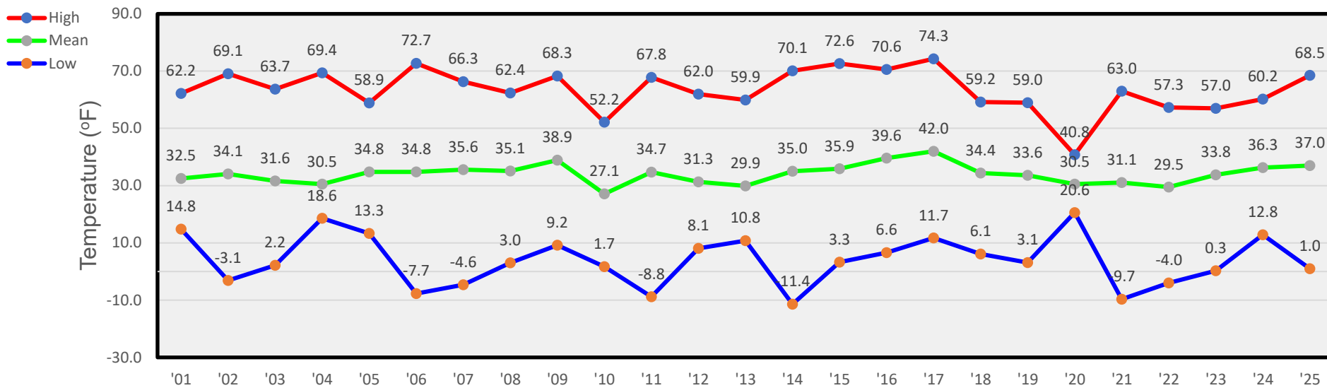
February Temperatures
