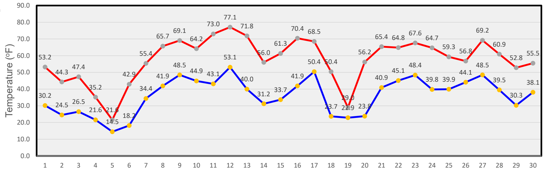
April Temperatures
