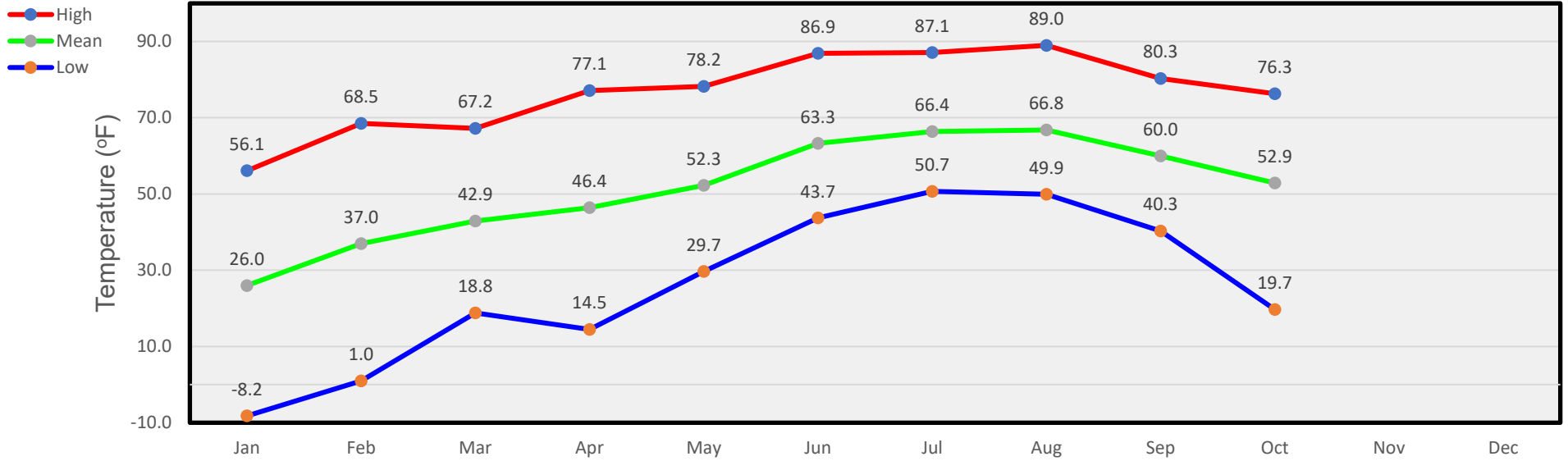
Monthly Temperatures
