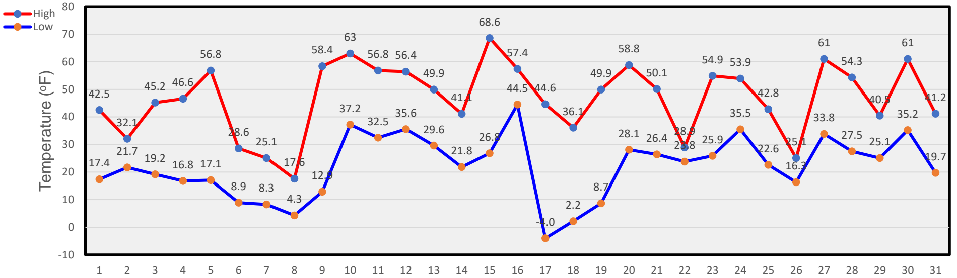
December Temperatures
