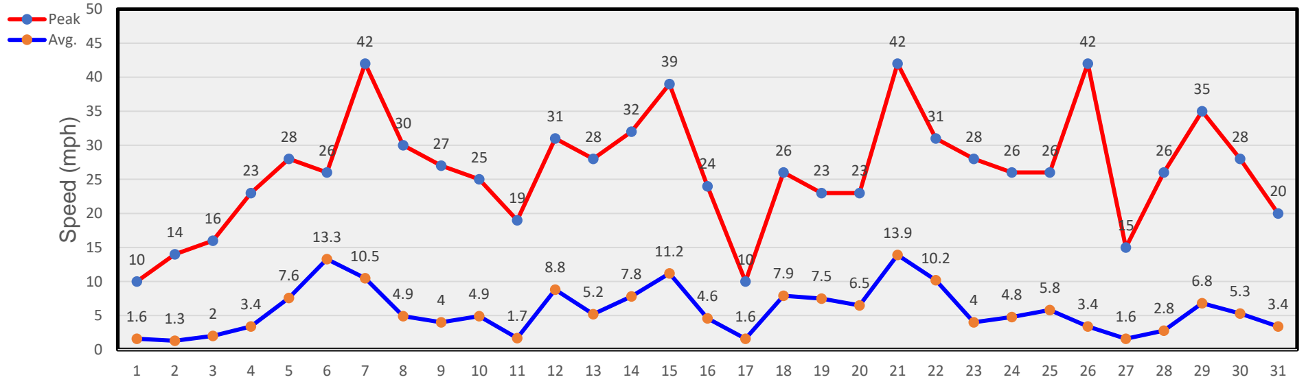
May Winds
