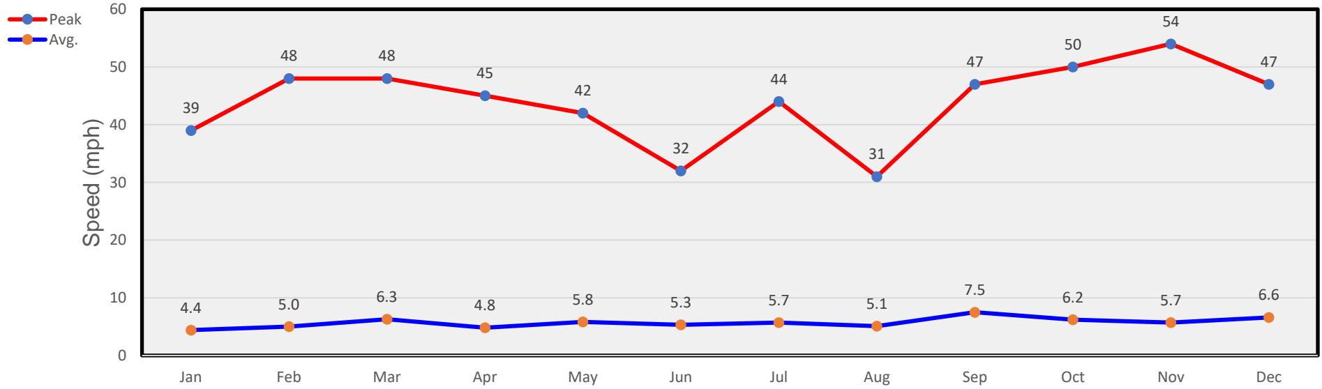
Monthly Winds
